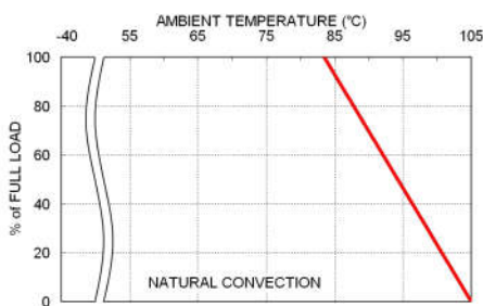
RED40-24S05W Derating Curve With Heat-sink
